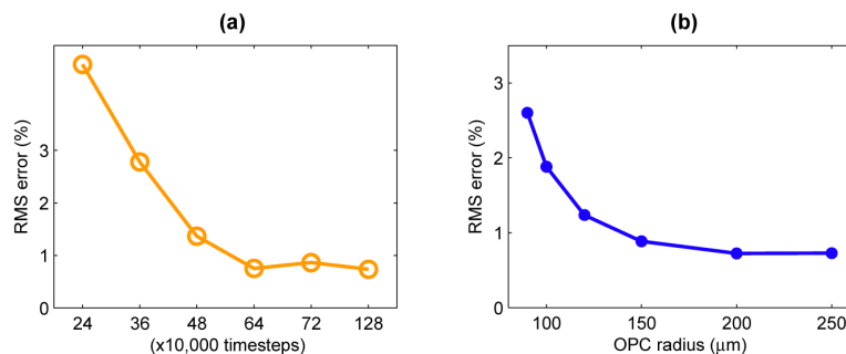
Fig. 9. Convergence analyses of the simulation. With a soft sink to eliminate the outgoing light component, the impinging light profile reconstructed from back-propagated light is compared to the original outgoing light in the forward scenario. The accuracy of the simulation increases with: (a) increased number of simulation time-steps (CW steady state), and, (b) increased distance between the OPC region and the scattering medium, where outgoing light impinges the OPC region at near normal incidence.
